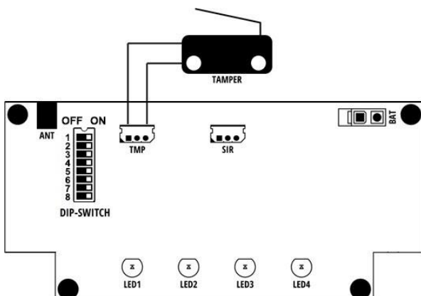
Figure 2 – Electronic board
